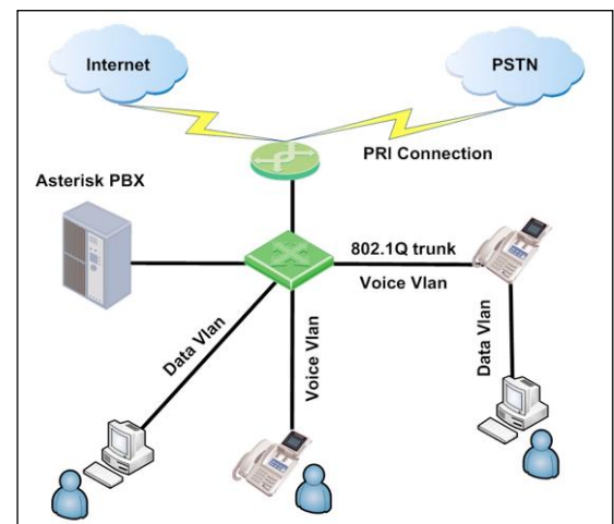
Figura 58: Asterisk PBX (Visio diagram by Amir Avraham)
